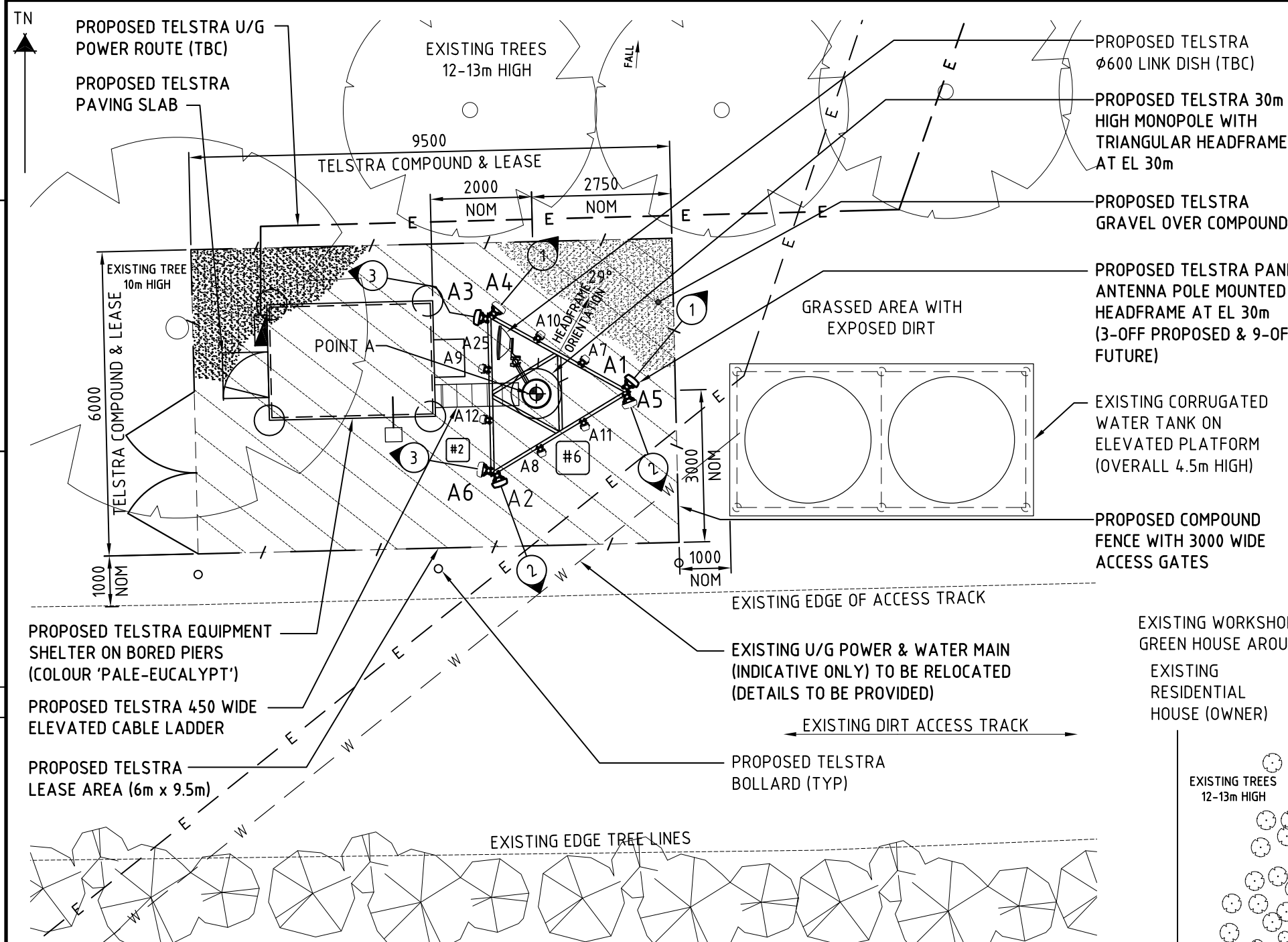
SITE LAYOUT SCALE 1:100
