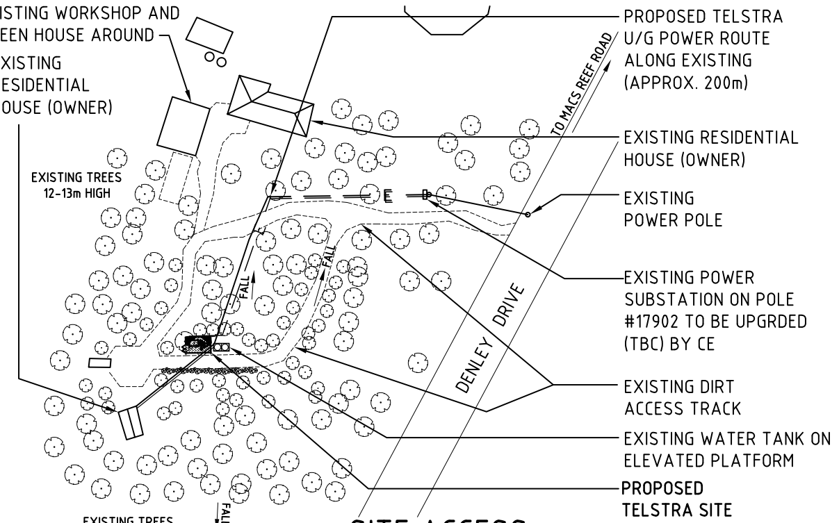
SITE ACCESS SCALE 1:2000
